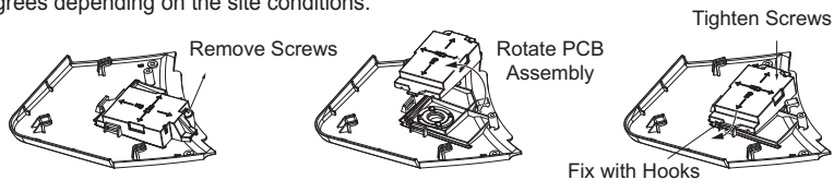
Figure. 90-degree Rotated Installation
