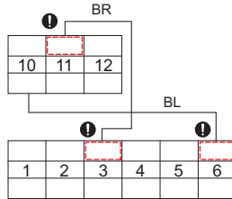
Terminal block 6 (In 3Ø Backup Heater)
