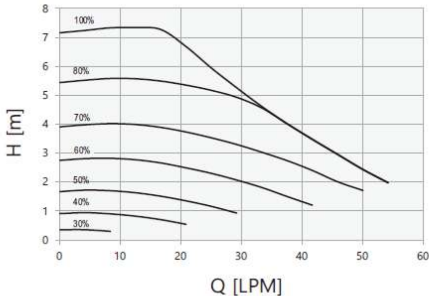
Q-H Chart
